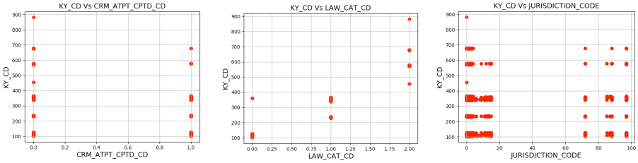
Figure 4: Linearity KY_CD
