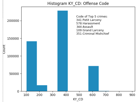
Figure 2: KY_CD
