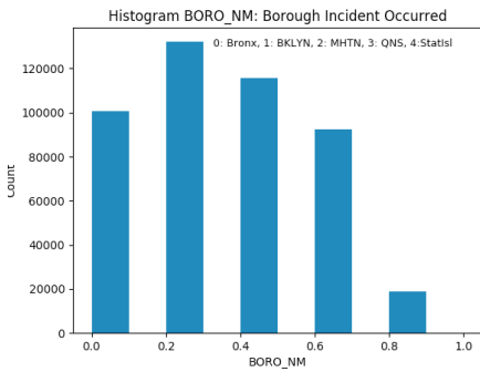
Figure 1: BORO_NM
