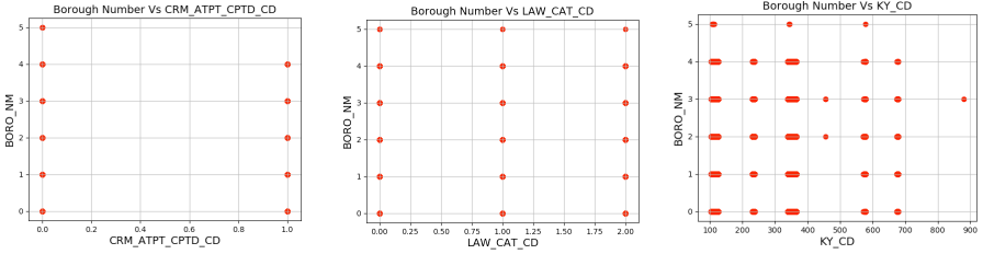
Figure 3: Linearity BORO_NM
