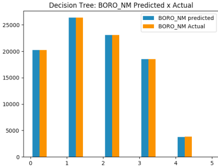
Figure 5: Decision Tree
